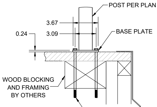
POST BASE CONNECTIONS INTO WOOD WITH THRU BOLTS
