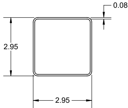
3" POST
