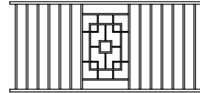
MOSAIC 71.75"x34"
