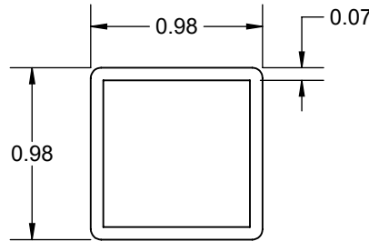
TOP / BTM RAIL
