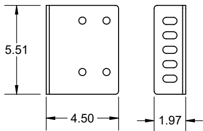
FASCIA BRACKET
