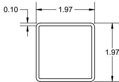
2" POST
