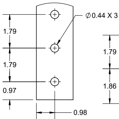
DETAIL B SCALE 1 : 3
