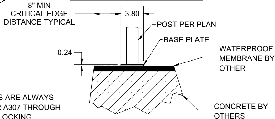
POST BASE CONNECTION INTO CONCRETE WITH WEDGE ANCHORS
