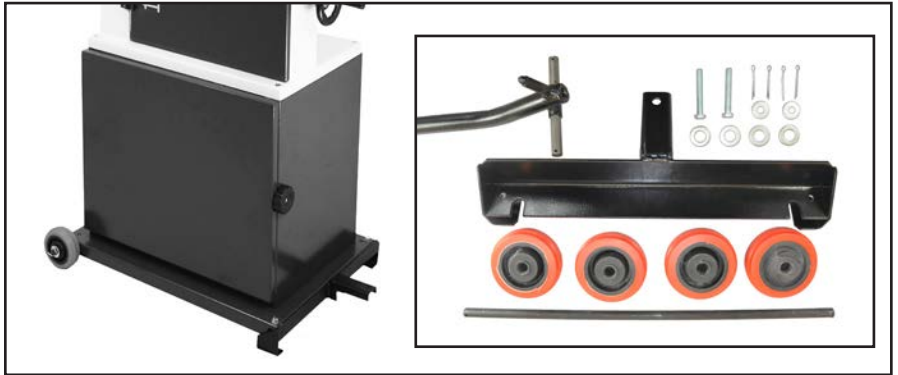
13-325 MOBILITY KIT Conversion Kit installs onto the bandsaw base to make it easy to move around the shop. Includes rear wheel assembly, front support, tow bar, hardware and instructions.
